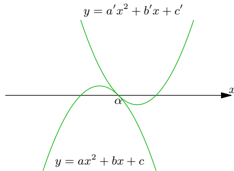
Figure 4.10 Common roots
