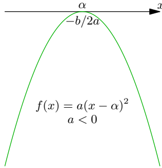
Figure 4.8 f(\alpha) = 0, f'(\alpha) = 0
