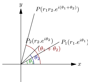
Figure 3.4 Complex numbers multiplication
