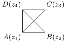
Figure 3.10 Square
