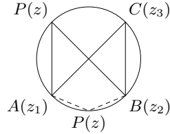
Figure 3.13 Circle through three points
