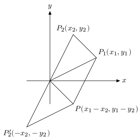
Figure 3.3 Complex numbers subtraction
