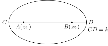
Figure 3.16 Locus of an Ellipse
