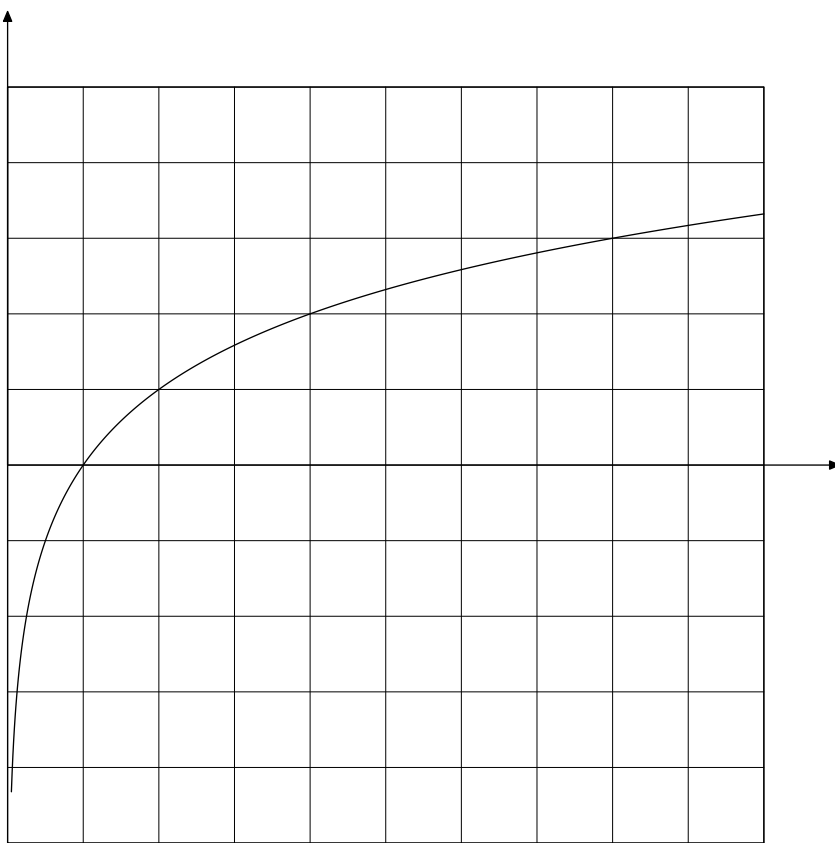
Figure 1.1 Graph of \log x .
