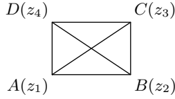
Figure 3.11 Rectangle
