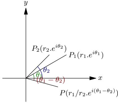
Figure 3.5 Complex numbers division
