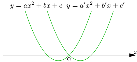
Figure 4.9 Common roots
