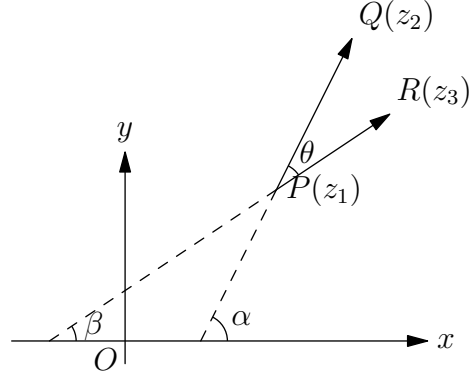
Figure 3.7 Angle relation between three complex numbers
